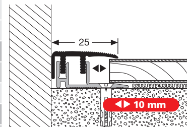
PF 587 L Maxx \updownarrow 8 - 12 mm
